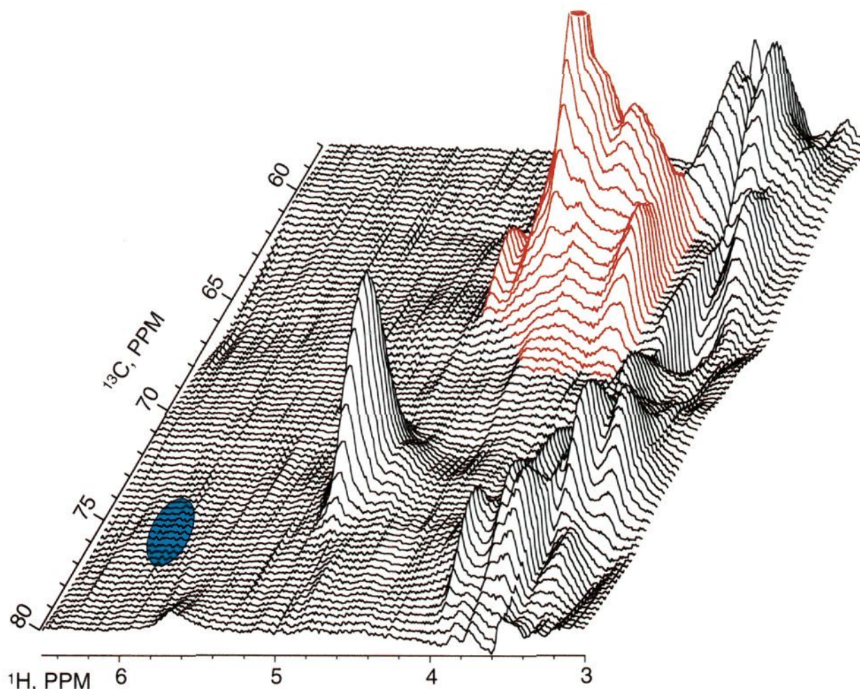
Figure 4. Stacked plot of the aliphatic region of the HMQC spectrum of D-LPC (same region as in Figure 3) showing the \gamma -ester correlations (red) and absence of \alpha -ester correlations (blue region) above the noise level.
