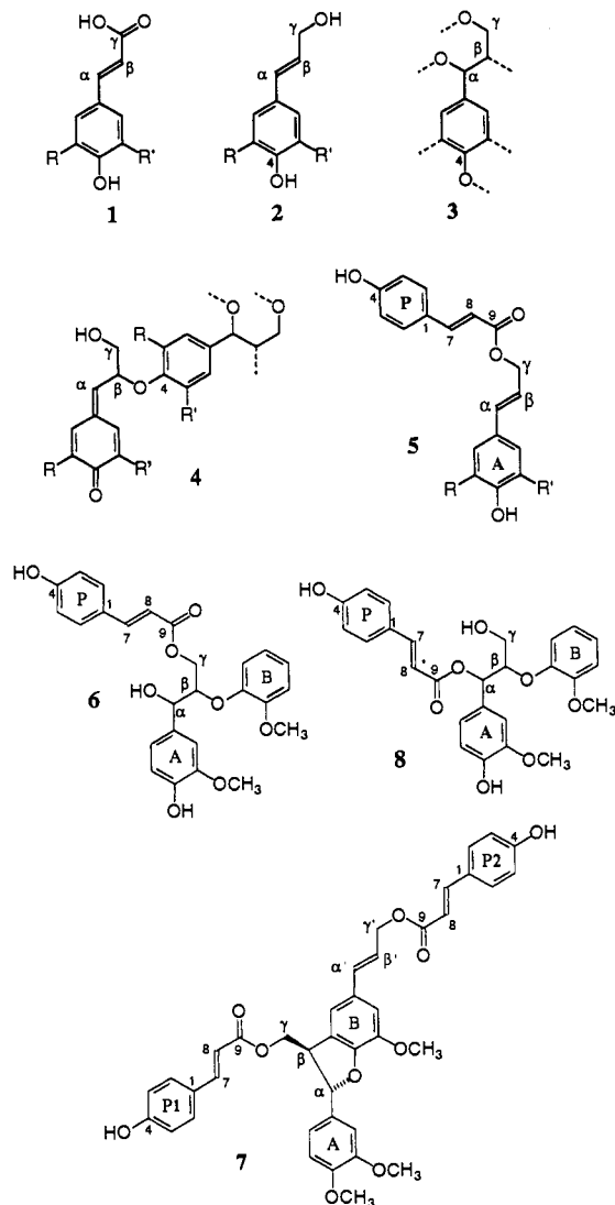
Figure 1. Plant cell wall precursors p -hydroxycinnamic acids 1 and monomeric p -hydroxycinnamyl alcohol lignin precursors 2 , a general structure of lignin 3 , quinone methide lignin intermediates 4 , p -hydroxycinnamyl p -coumarates 5 , and \alpha - and \gamma - p -hydroxycinnamate ester model compounds 6–8 synthesized for NMR correlation work. For compounds 1 , 2 , 4 , and 5 , (a) R = R' = H; (b) R = OCH 3 , R' = H; and (c) R = R' = OCH 3 .
